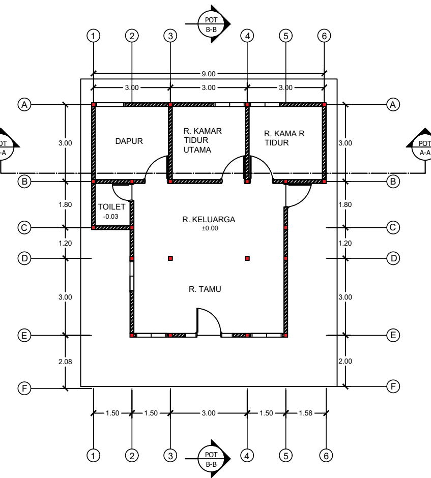
DENAH TYPE 80 0 1 2 3 4 5
