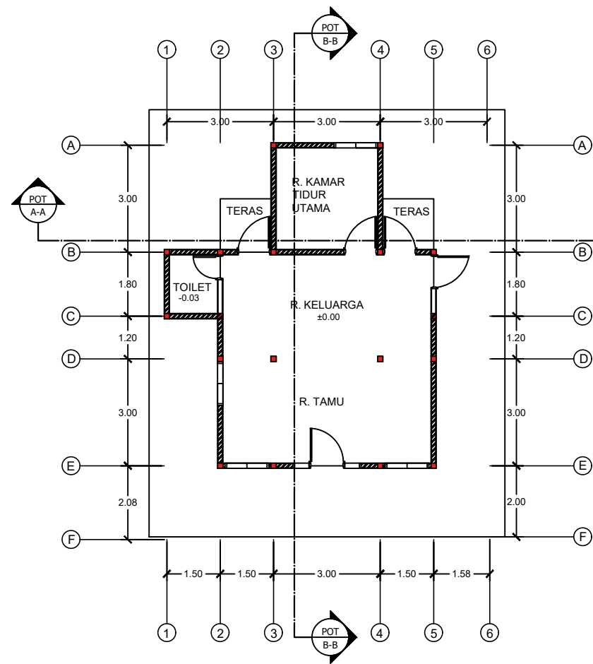
DENAH TYPE 60 0 1 2 3 4 5
