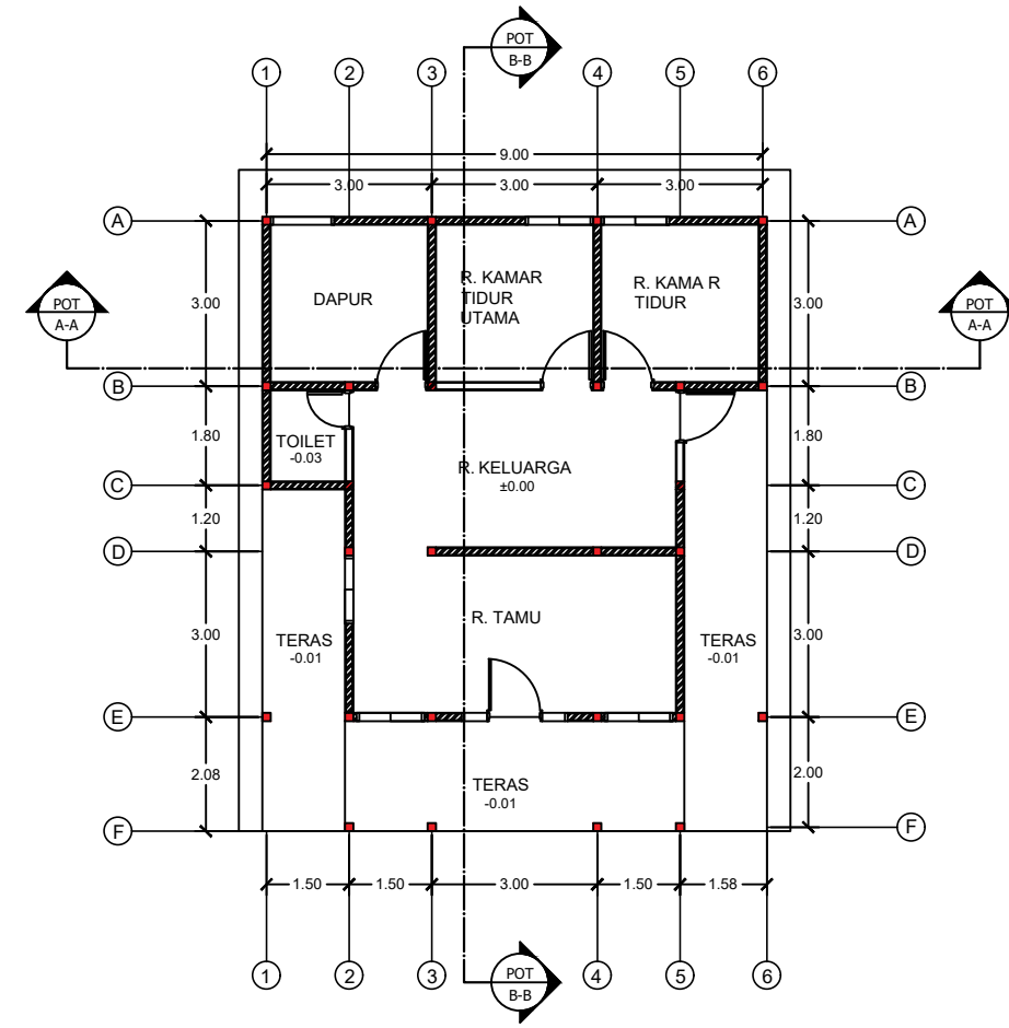
DENAH TYPE 90 0 1 2 3 4 5
