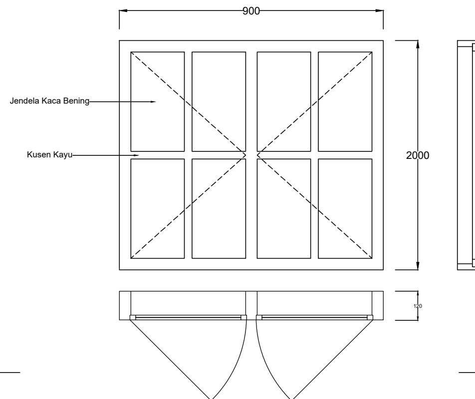
DETAIL JENDELA J2 1 : 20
