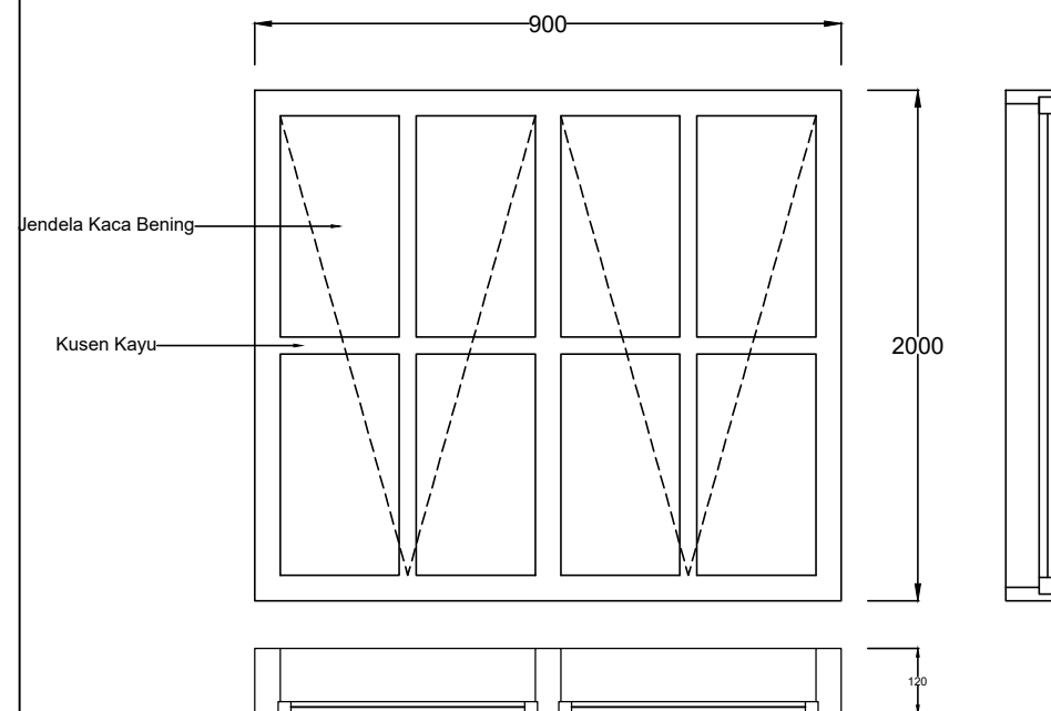
DETAIL JENDELA J2 1 : 20
