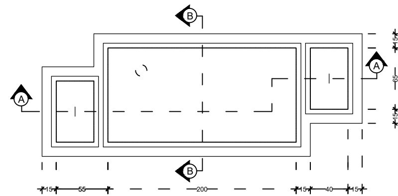
DETAIL SEPTICTANK SKALA 1 : 40
