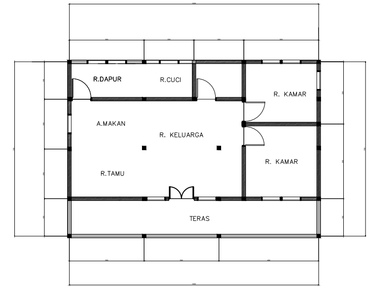
DENAH TYPE 70 0 1 2 3 4 5
